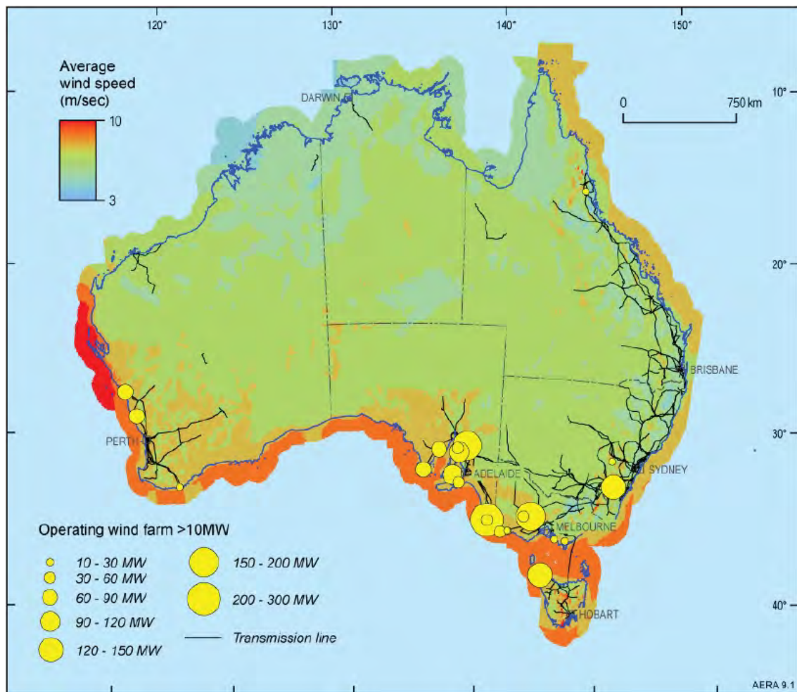
Figure 1-2 Australia wind resources
