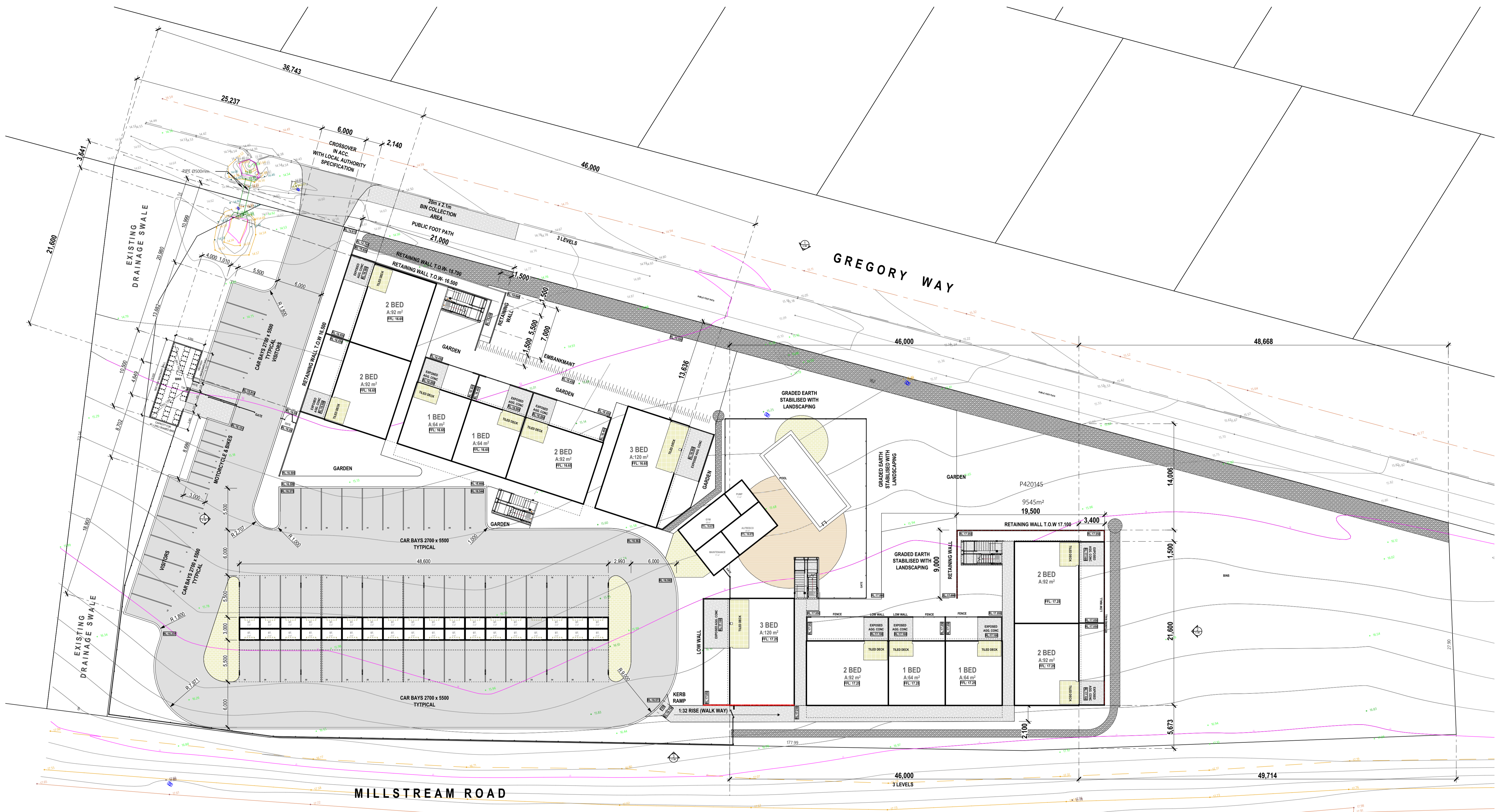
-1. SITE PLAN #LayerID Scale 1:250
